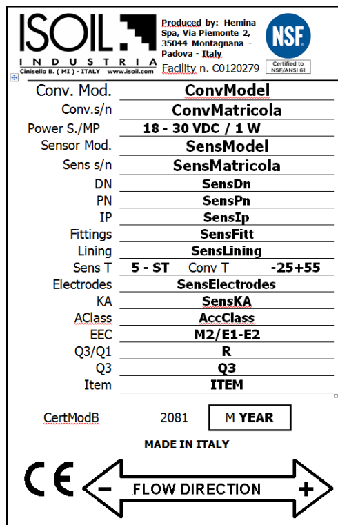
Figure 2 – Metrological label MV800 – Sensor MS2500
